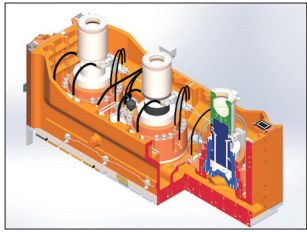
滑座快速上昇装置 Quick lift slide device
